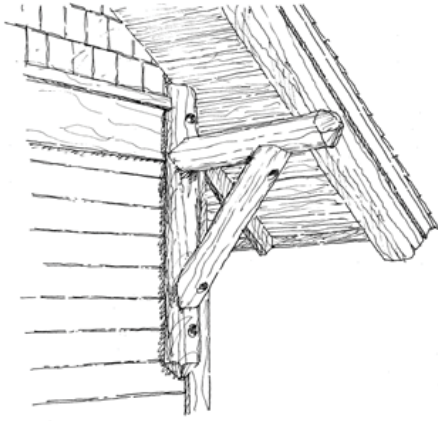
Log knee brace supporting roof
